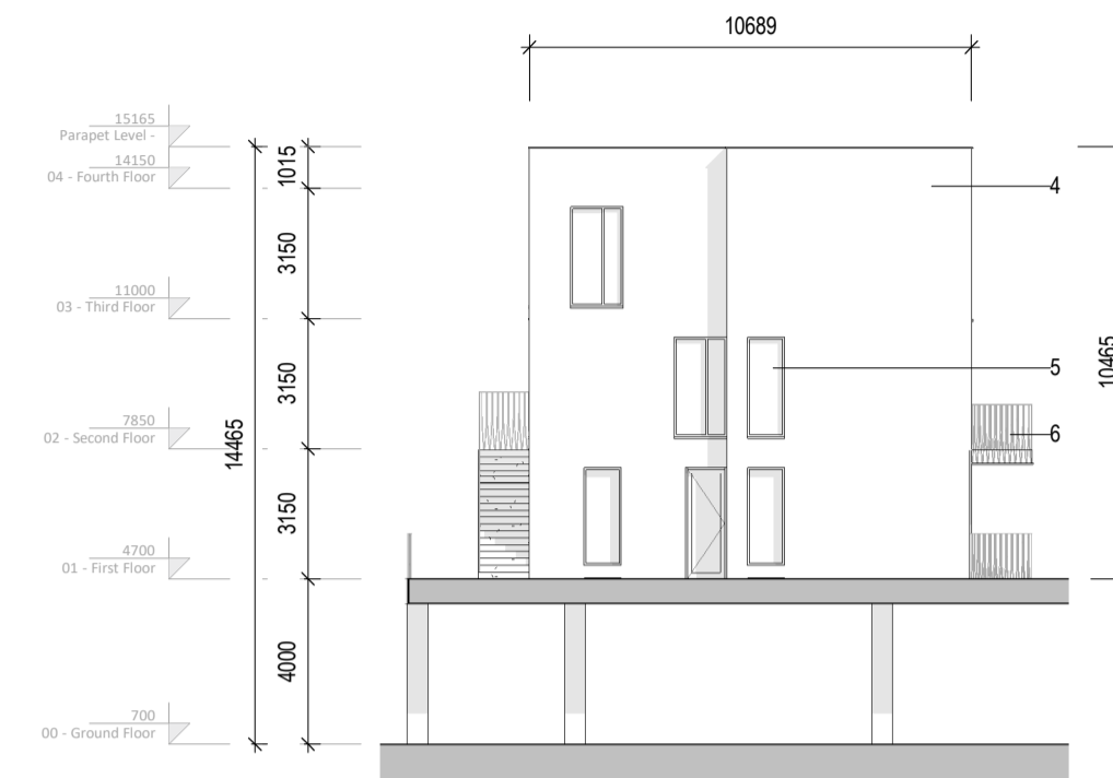
3 A1 Duplex North-West Elevation 1:200
