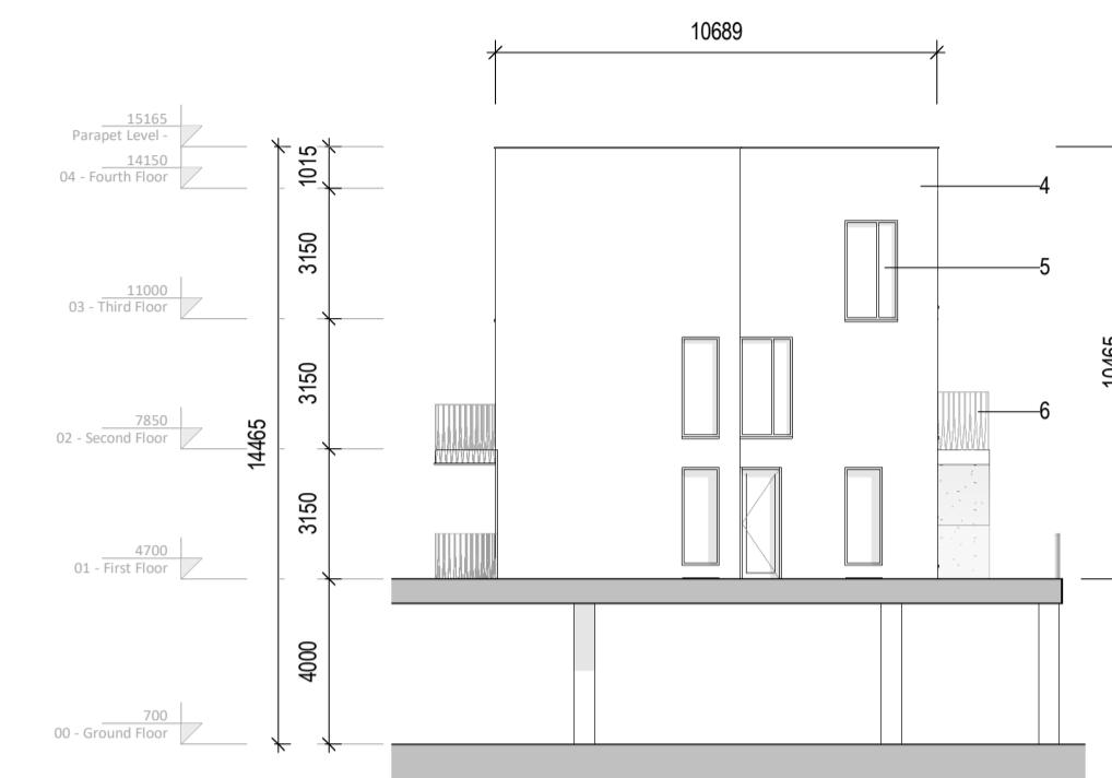
4 A1 Duplex East-South Elevation 1:200
