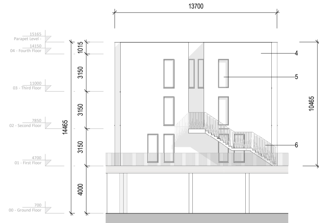
2 A1 Duplex North-East Elevation 1:200
